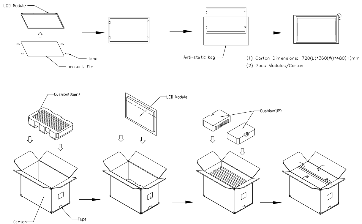
Figure. 7-1 Packing method
